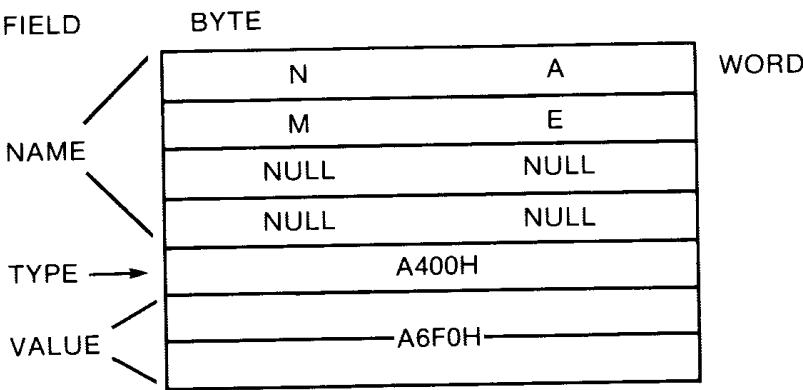
Figure 3-3. Entry in Symbol Table
