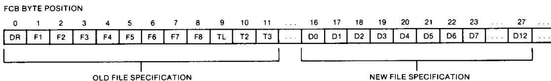
Figure 4-1. FCB Format for Rename Function
