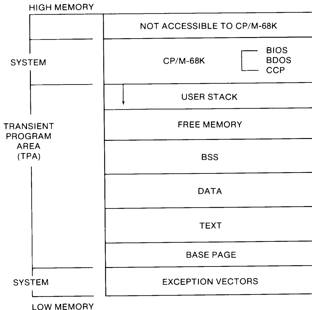
Figure 2-3. CP/M-68K Memory Model with Inaccessible Memory
