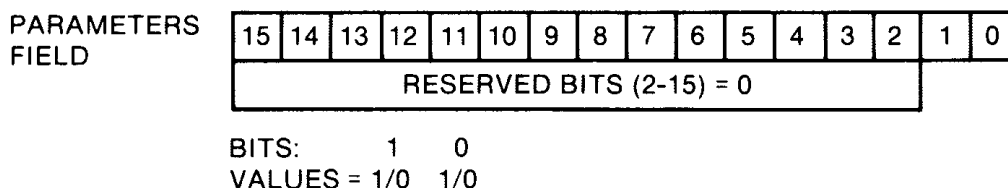
Figure 4-9. Parameters Field in TPAB
