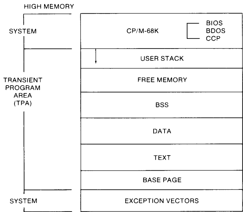
Figure 2-2. CP/M-68K Default Memory Model
