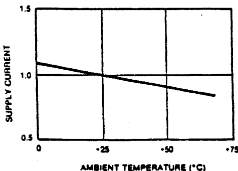
Typical Supply Current vs. Temperature, Normalized
