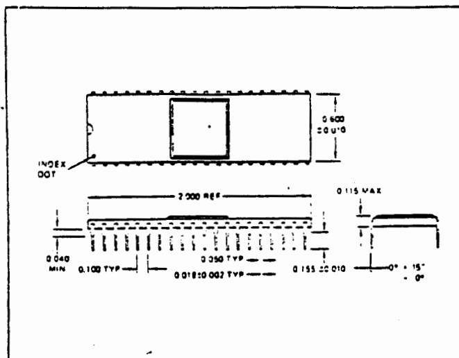
WD8250 CERAMIC PACKAGE
