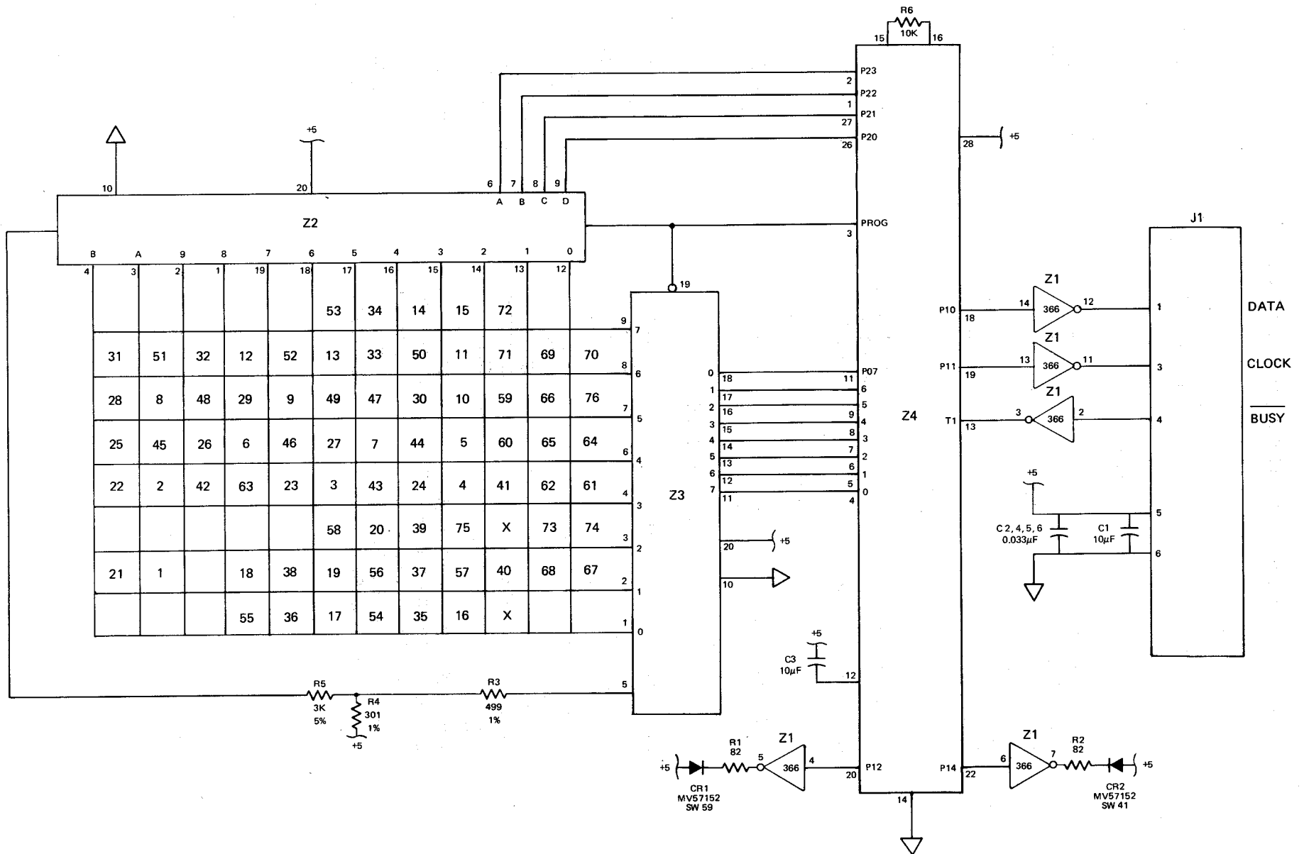
Figure 4. Keyboard Schematic Diagram
