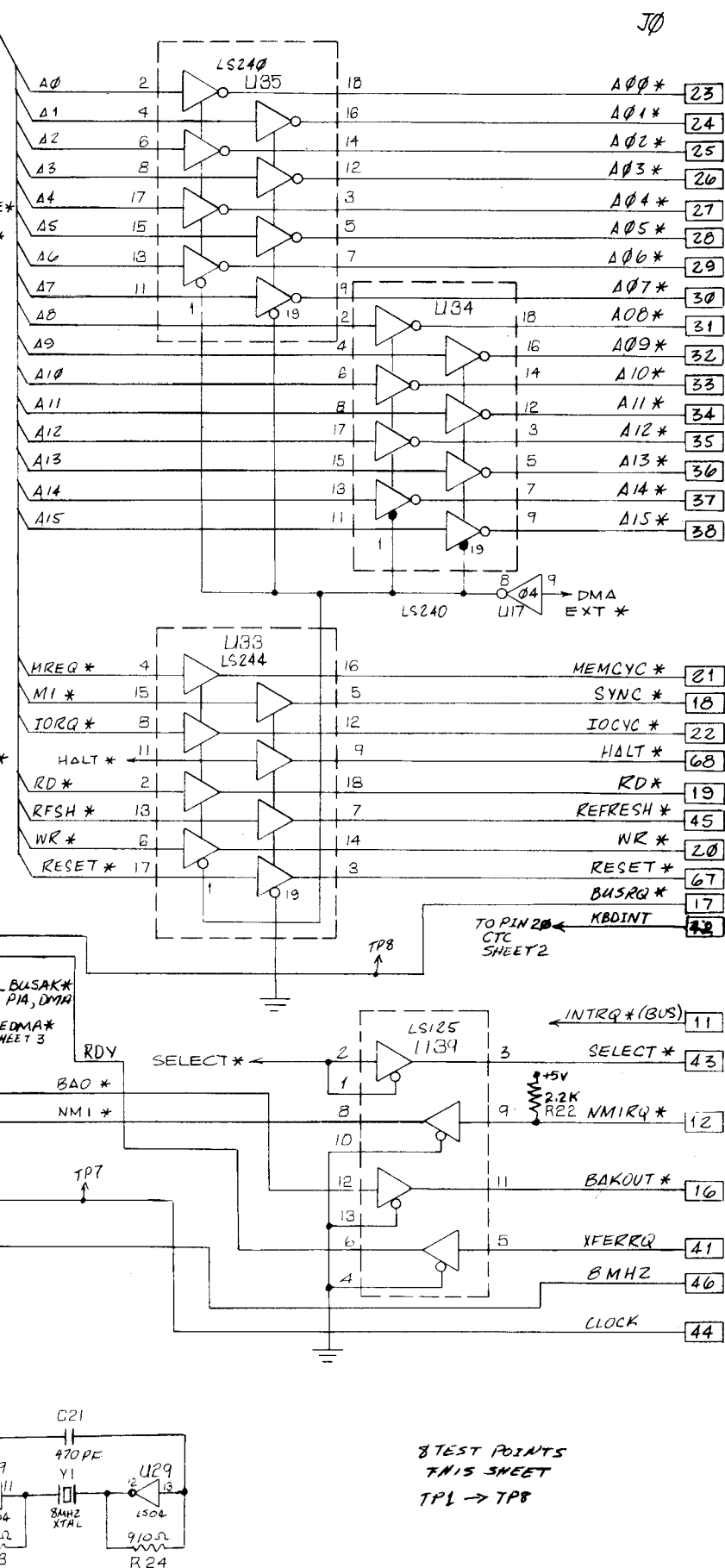
Schematic Diagram — Sheet 1
