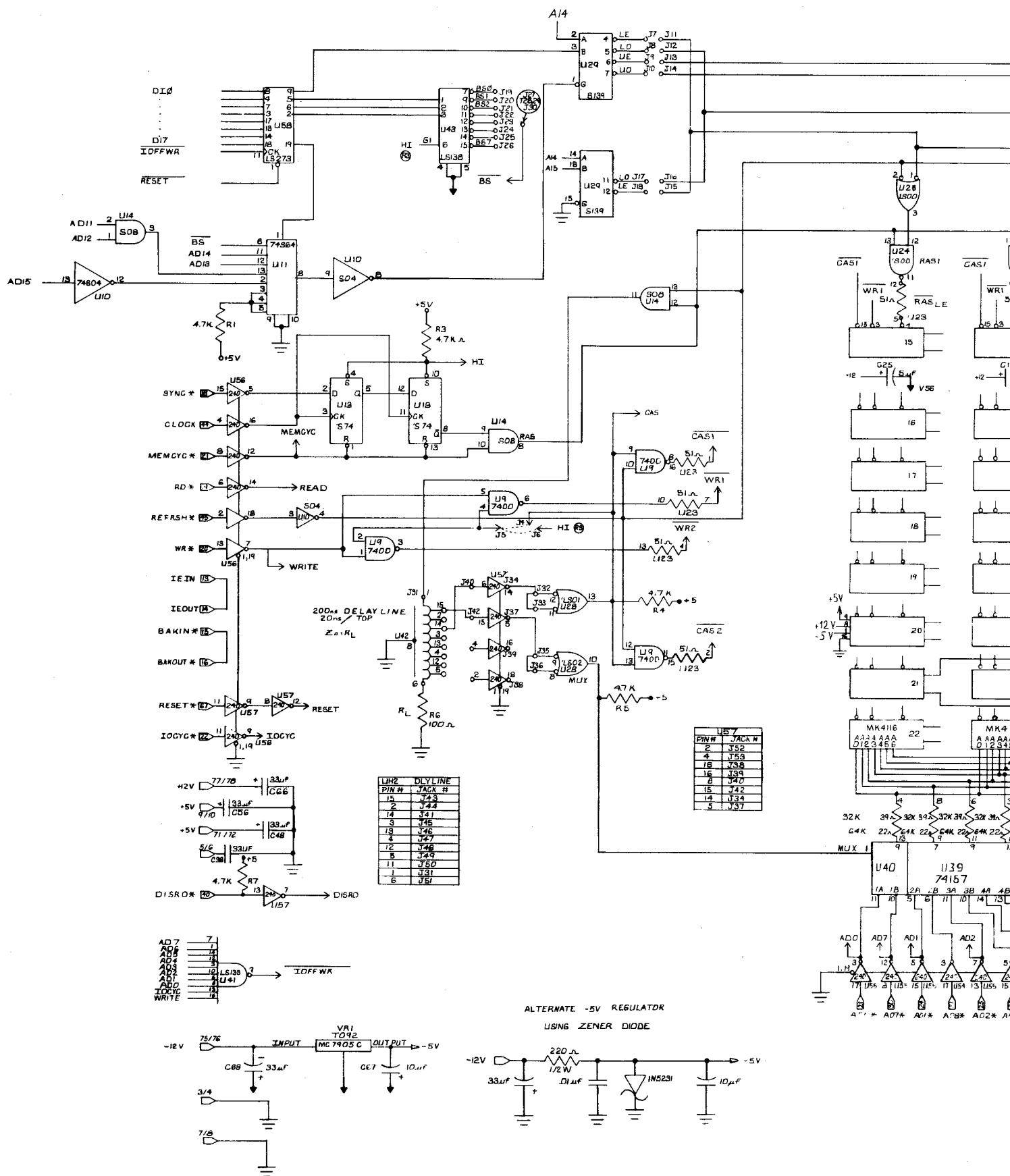
Figure 5. Memory Board
