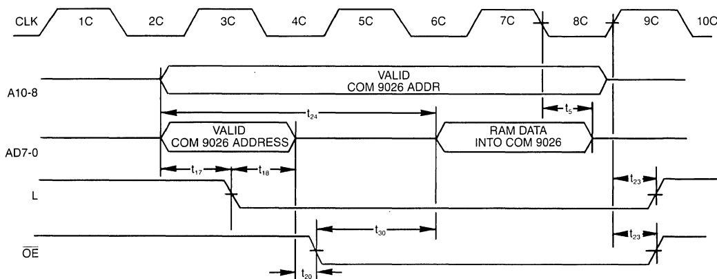
FIGURE 15—COM 9026 READ RAM AC TIMING
