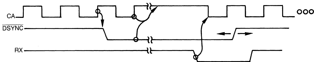
FIGURE 9—CA CLOCK GENERATOR TIMING
