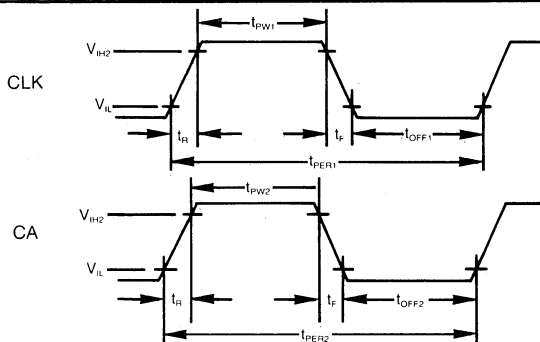
FIGURE 10— CLK, CA AC CHARACTERISTICS
