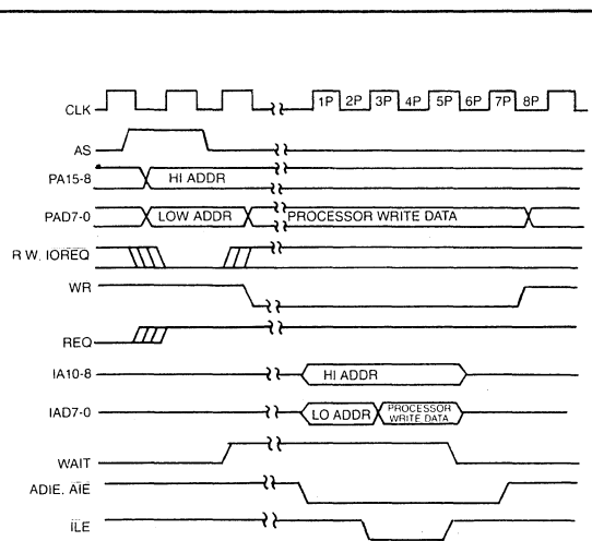
FIGURE 7—PROCESSOR WRITE COM 9026
