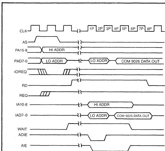
FIGURE 6—PROCESSOR READ COM 9026
