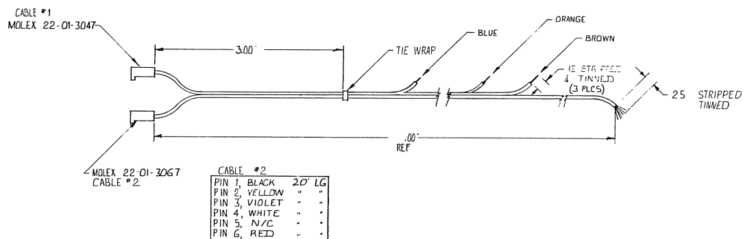
LED Driver Board Harness (Secondary)
