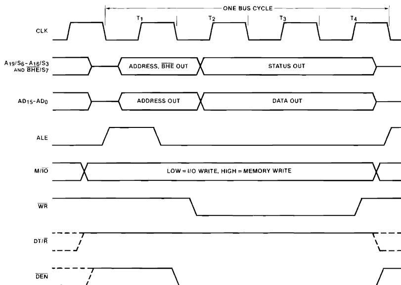
Figure 4-8. 8086 Write Bus Cycle
