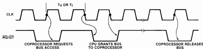
Figure 4-16. Request/Grant Timing
