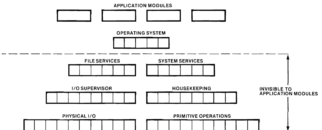
Figure 2-69. Operating System Hierarchy
