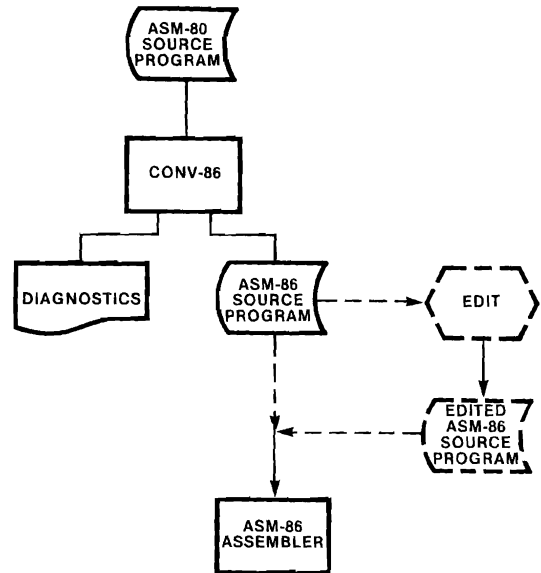
Figure 2-65. ASM-80/ASM-86 Conversion
