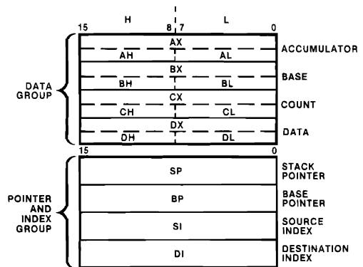
Figure 2-7. General Registers
