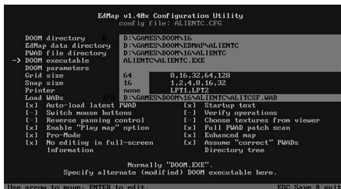
Listing 2.1. A sample ADD file: ALIENTC.ADD.
