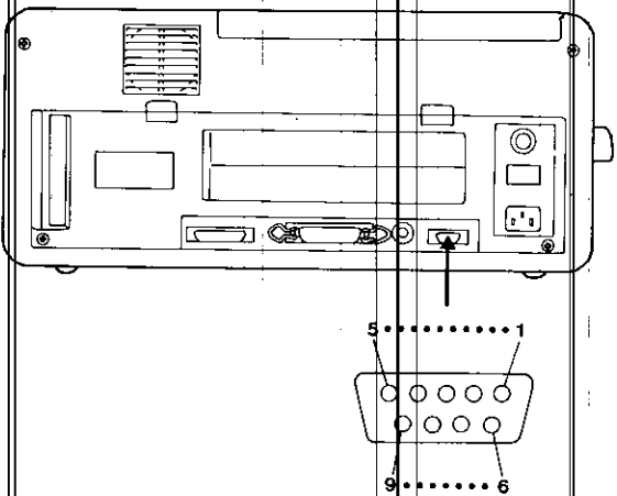
Fig. C-1. PIN ARRANGEMENT FOR RGB MONITOR
