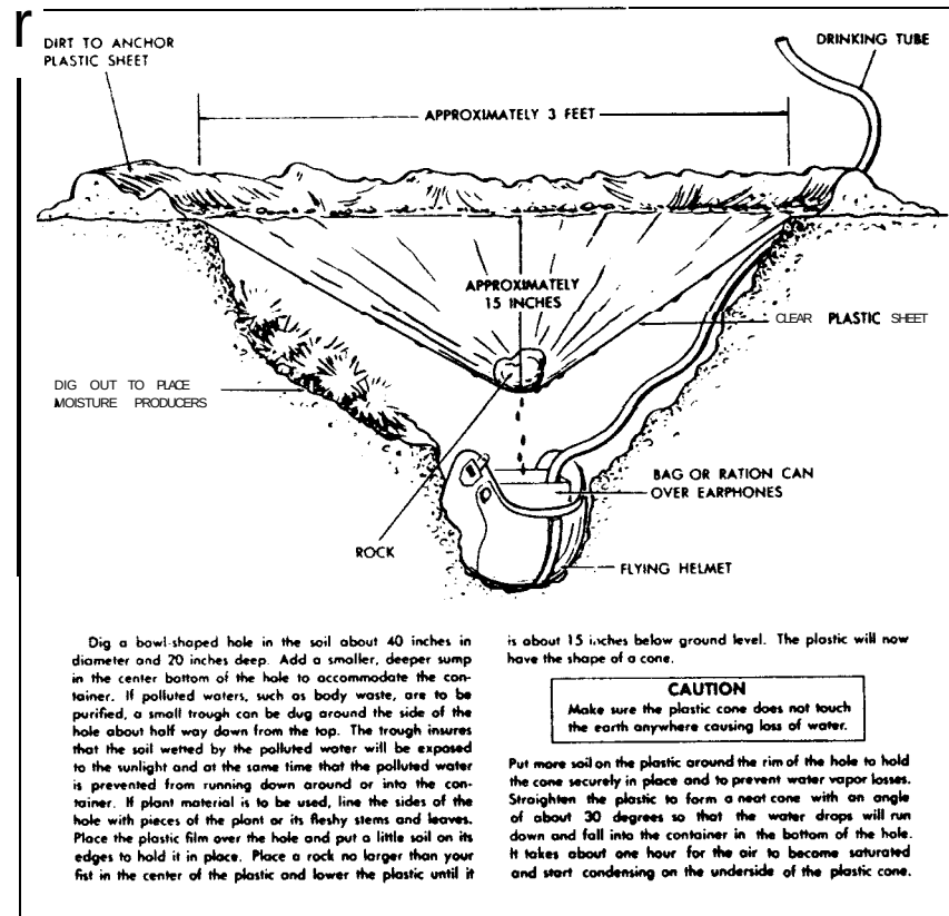
Figure 32: Cross Section of a Solar Still
